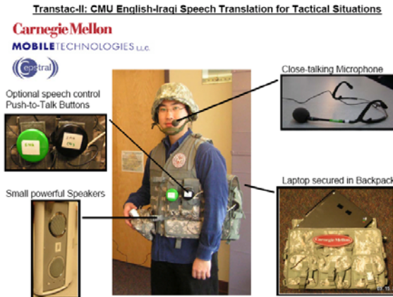
Figure 2: Hardware components
